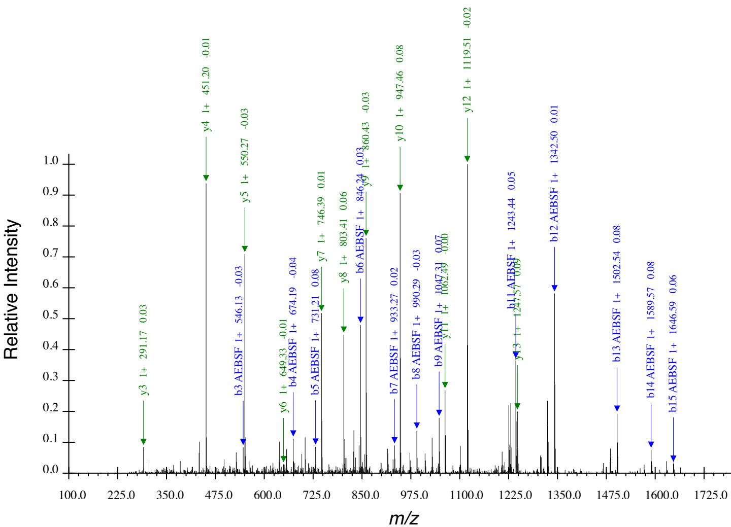
Trypsin's S195 labelled by AEBSF, z=2 , Mp/z^{\text{exact}} = 896.8509 Mp/z^{\text{obs}} = 896.8477 , \Delta MZ = -0.0033 , RT = 29.20 min, File: TC_03Dec17_R1
